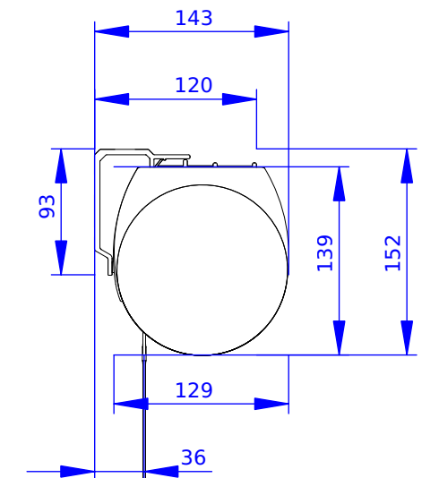
Case Side Detail
